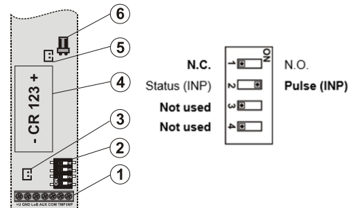
Fig. 2 – Transmitter JA-150TX-VX1: 1 – wire terminals, 2 – settings DIP switch (pre-set from factory, see picture), 3 – external tamper contact jumper, 4 – battery holder, 5 – external antenna jumper, 6 – external antenna connector
